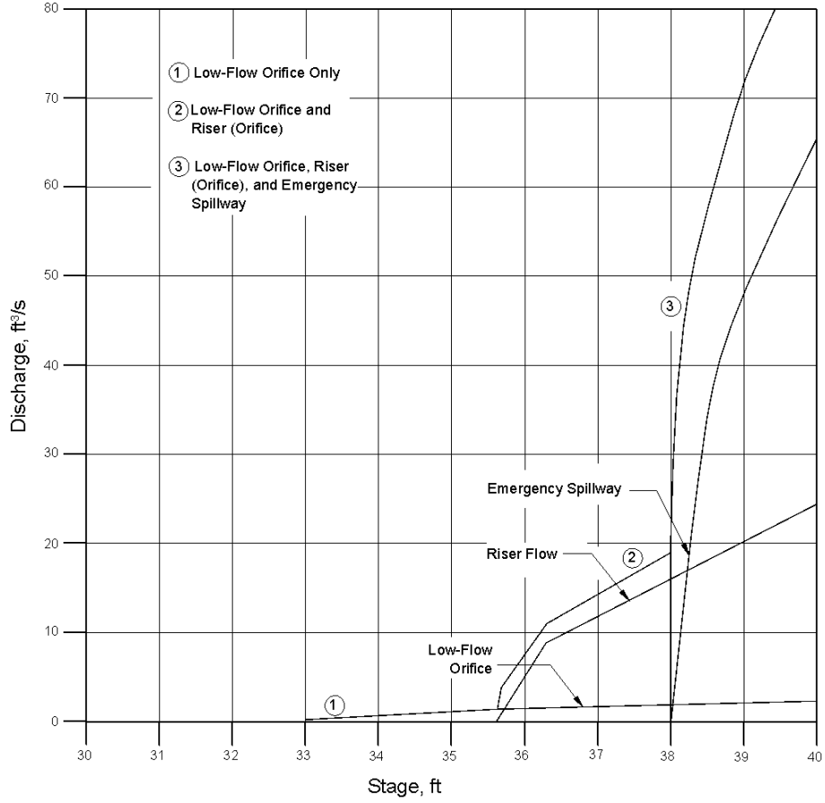
Figure Error! No text of specified style in document..4 Combined Stage-Discharge Relationship
