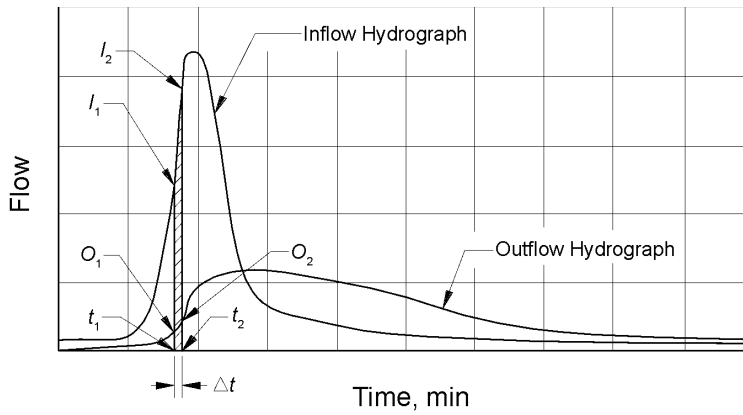
Figure 12.5 Routing Hydrograph Schematic
