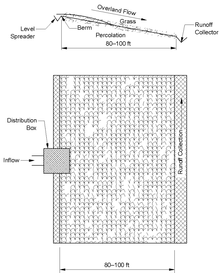
Figure Error! No text of specified style in document..14 Level Spreader System
