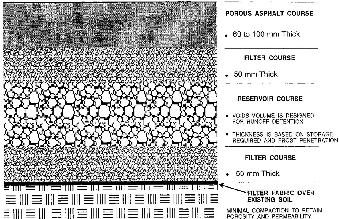
Figure 12.16 Porous Pavement
