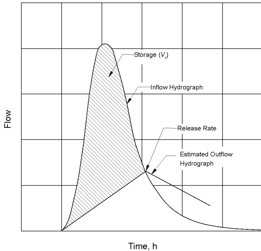
Figure Error! No text of specified style in document..3 Inflow and Outflow Hydrographs from a Stream Reach
