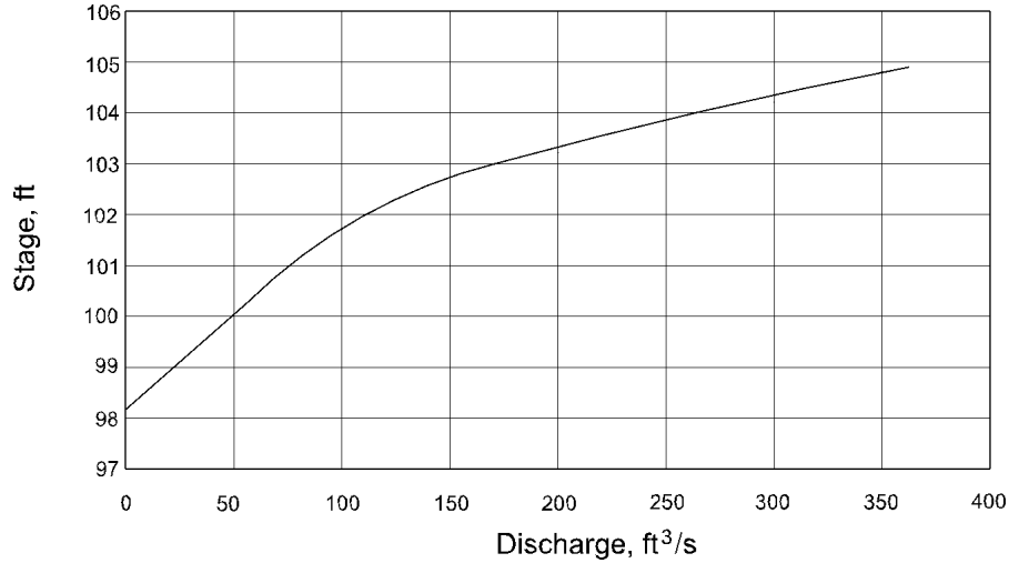
Figure 12 Error! No text of specified style in document..2 Example Stage-Discharge Curve
