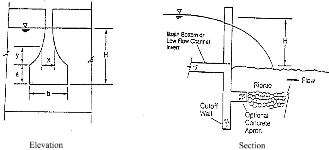
Figure 12.10 Proportional Weir Dimensions
