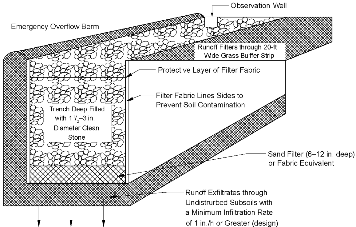
Figure 12.12 Infiltration Trench
