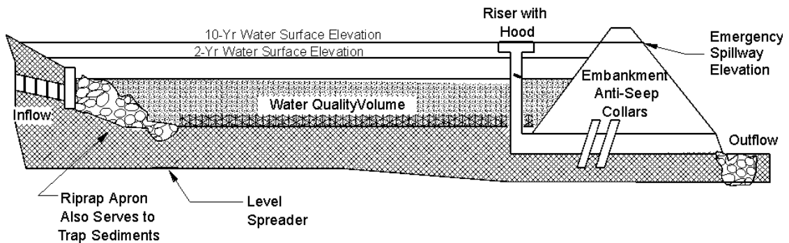
Figure 12.13 Infiltration Basin, source: Schueler
